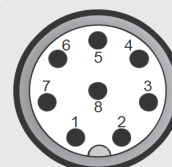
M12x1, 8 pole
